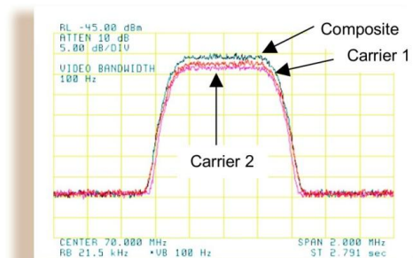
Figure 2: Duplex Link with DoubleTalk Carrier-in-Carrier
