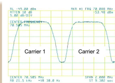
Figure 1: Traditional Full Duplex Link
