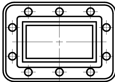
WR229 CPRG FLANGE PATTERN TYPICAL BOTH ENDS
