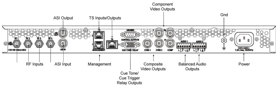
Figure 2. Cisco D9824 Rear Panel
